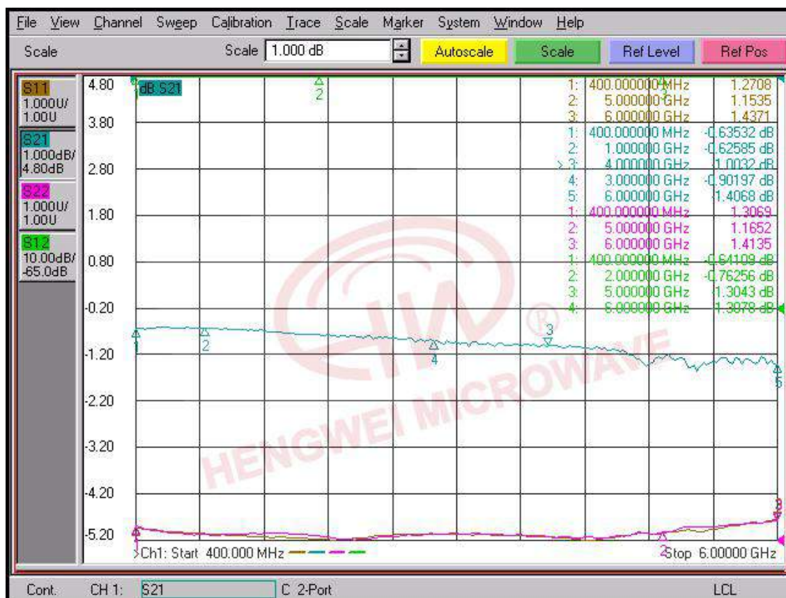
PIC1: INSERTION LOSS
